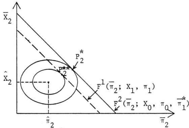
Figure 3 Optimal Second-Period Policy in a Two-Period Model
