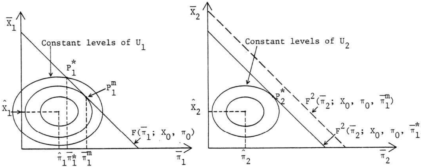
Figure 2 Optimal First-Period Policy in a Two-Period Model
