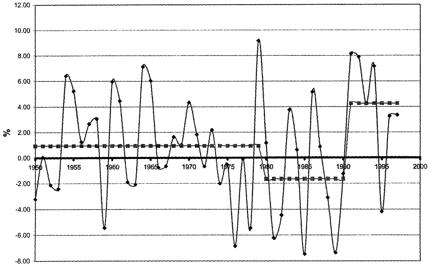
CHART 4 TFP GROWTH
