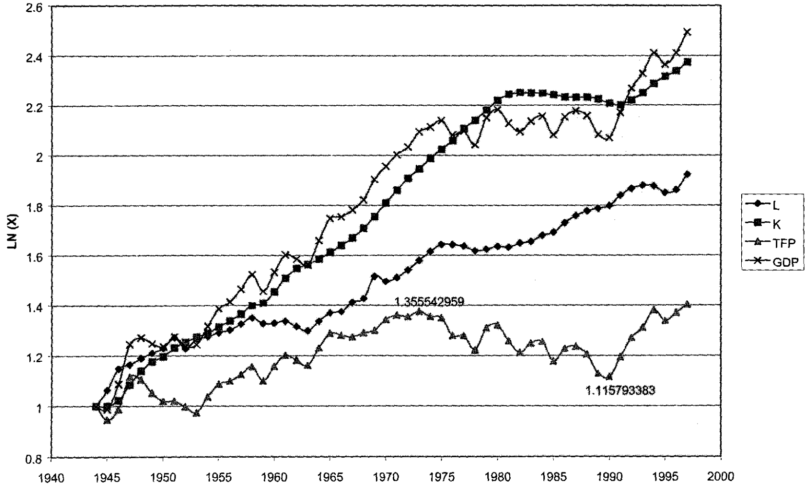
CHART 6 Growth accounting
