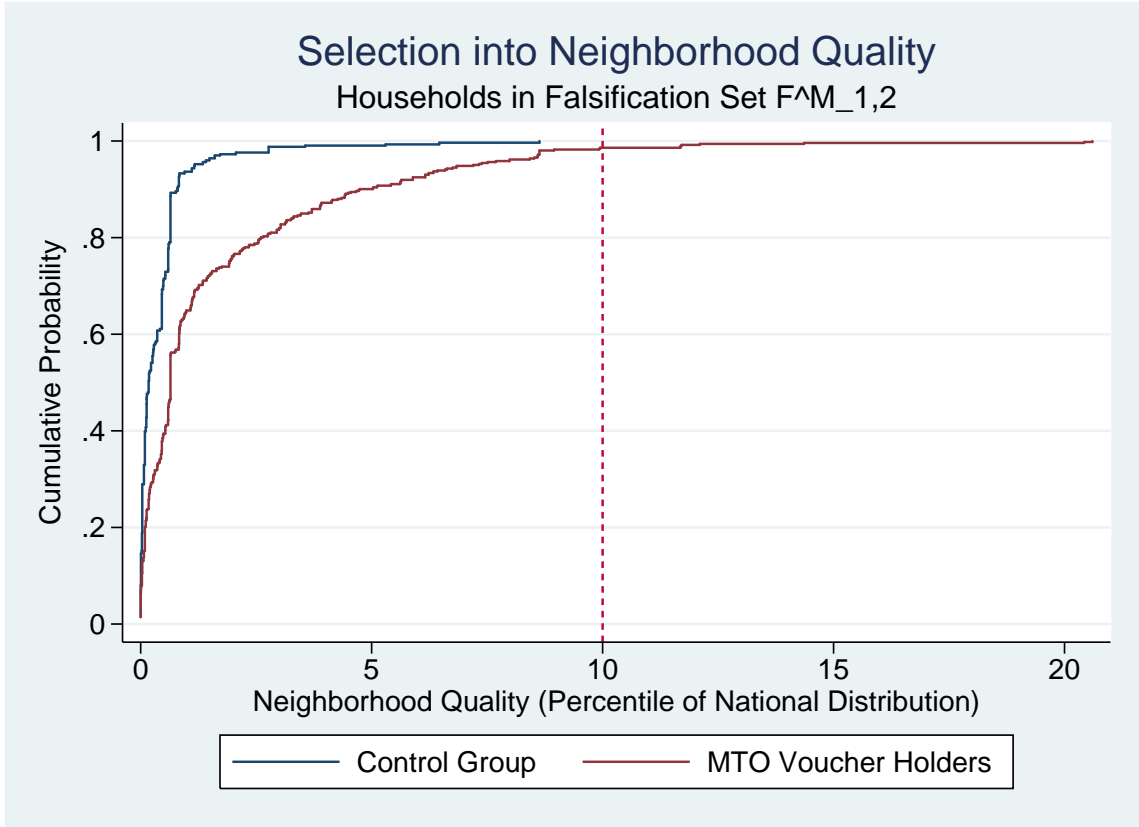
(b) Falsification Set F^M_{1,2}
