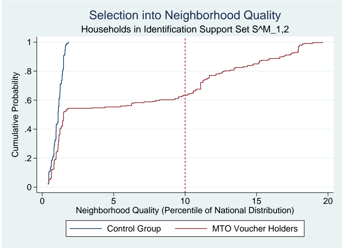
(a) LATE Identification Support Set S^M_{1,2}
