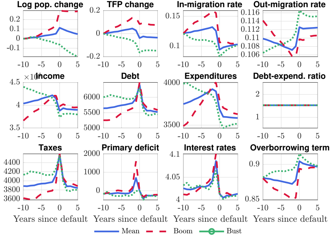
Figure 10: Default episodes
