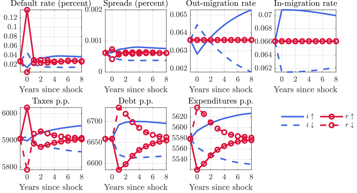
Figure 8: Model mechanisms
