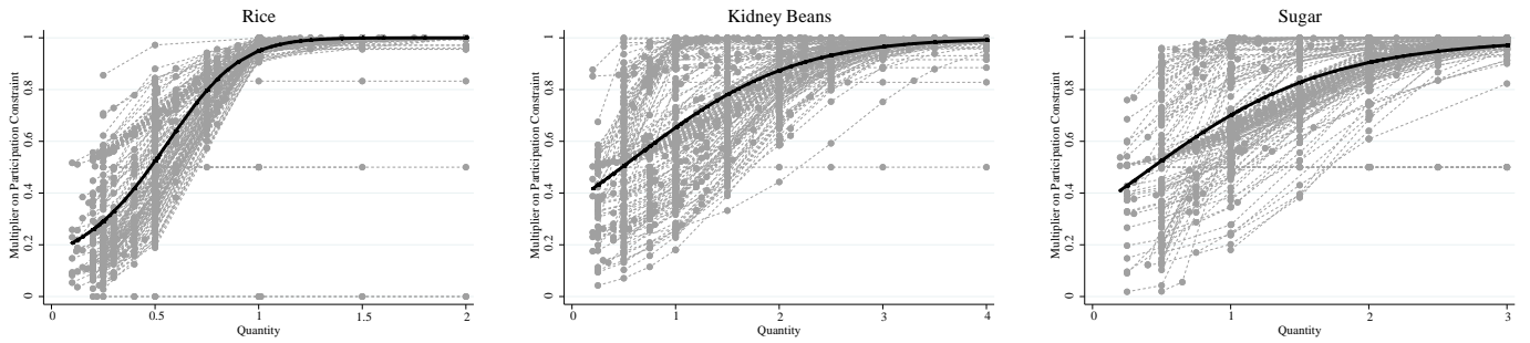
Figure 2: Estimated Multipliers on Participation (or Budget) Constraints
