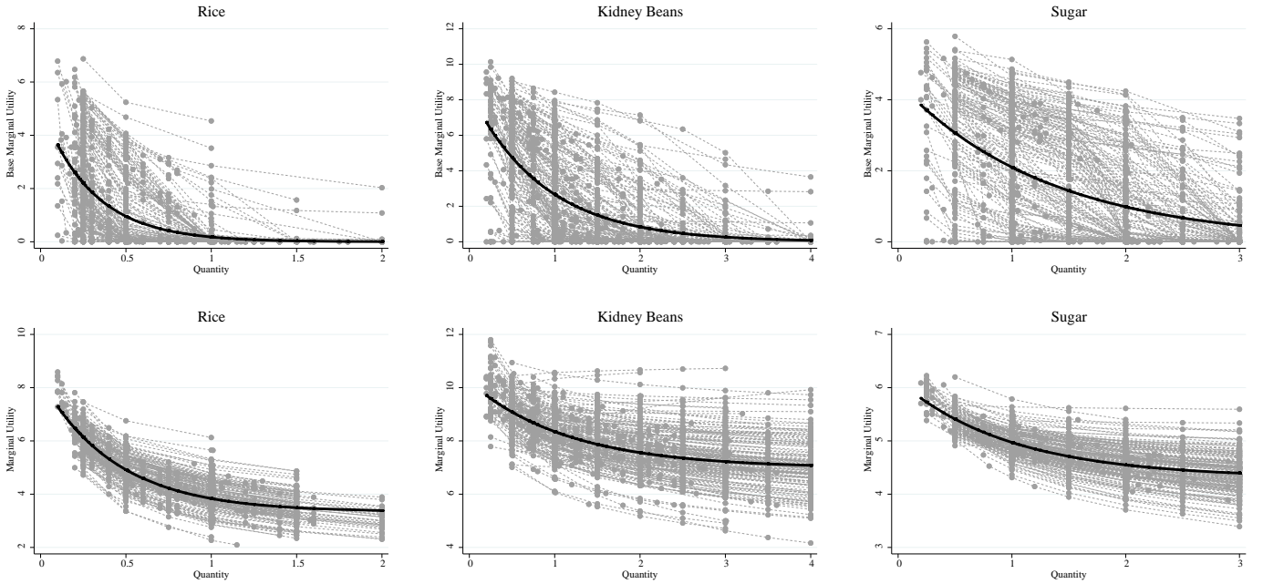
Figure 3: Estimated Base Marginal Utility (Top Panels) and Marginal Utility (Bottom Panels)
