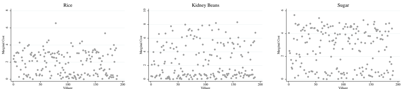
Figure 5: Estimated Marginal Cost
