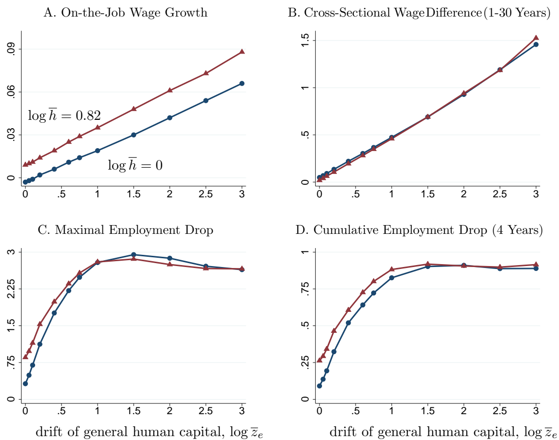
Figure 9: Robustness Analysis
